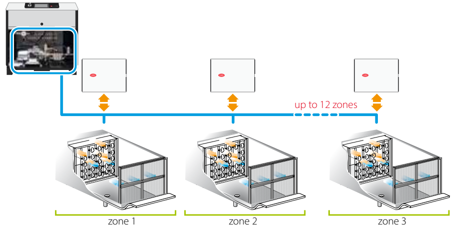
Example of a multizone system with one pumping station and one zone control unit
